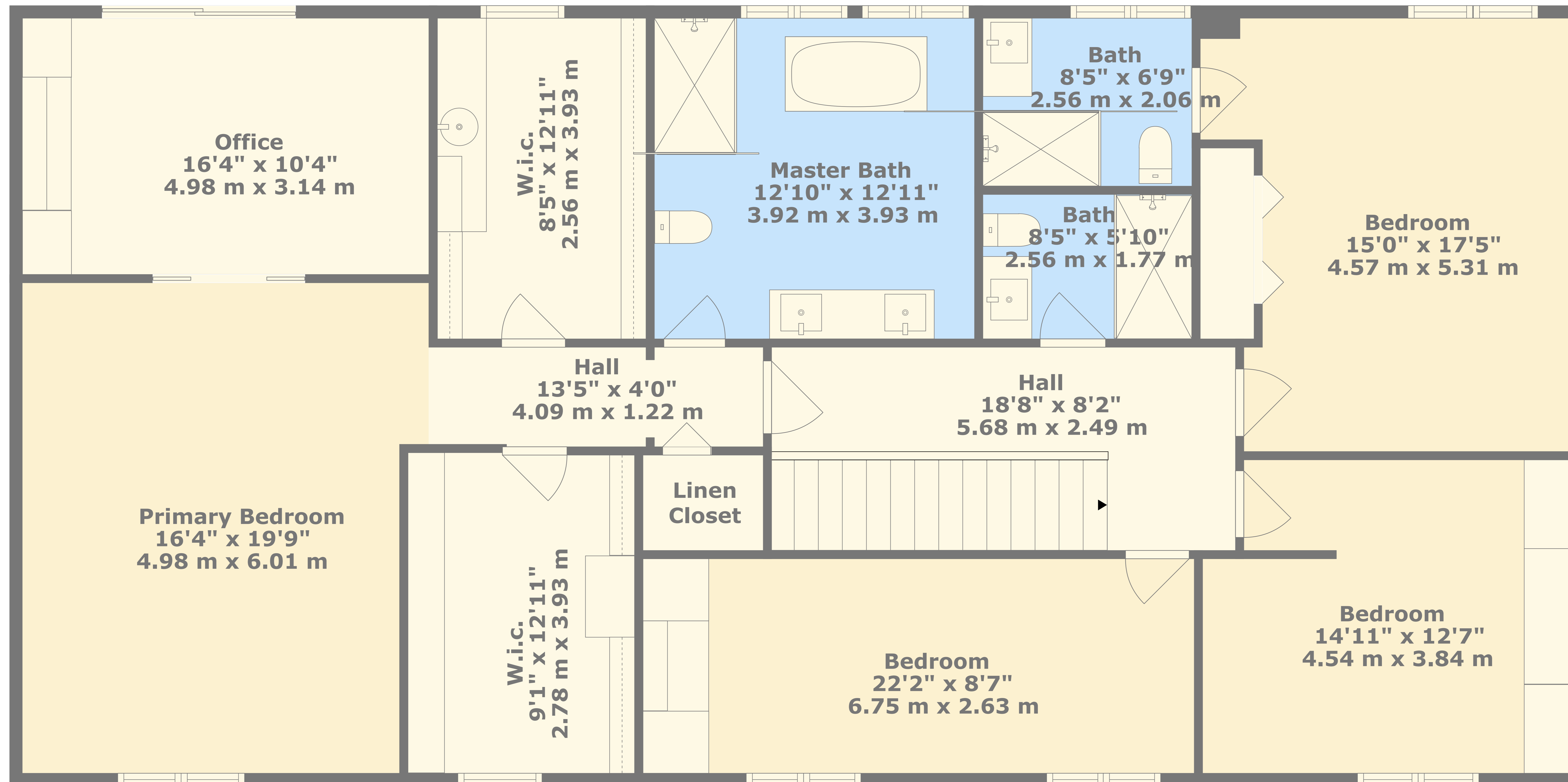
Floor 2
